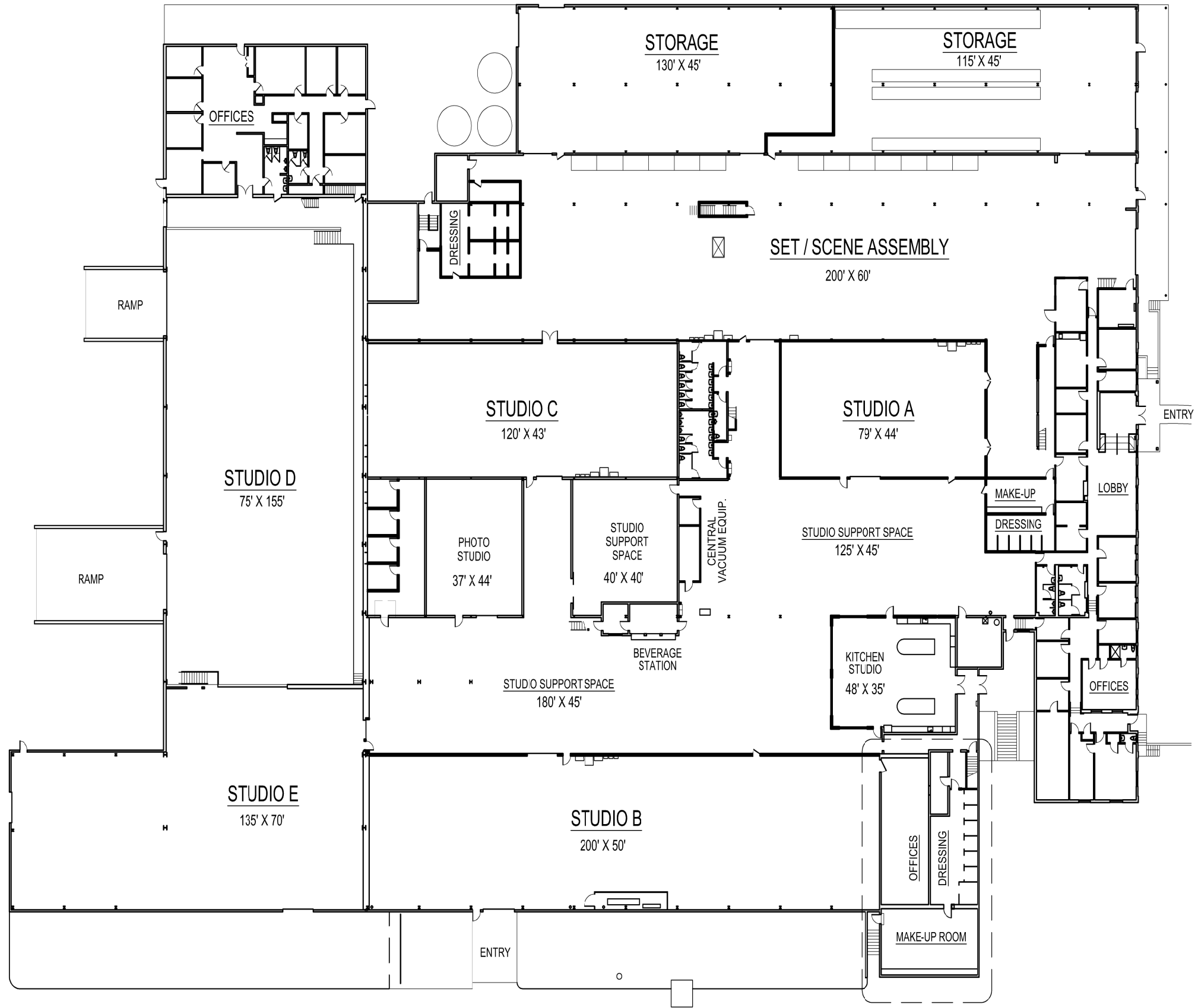
3 RIVERS STUDIOS - MAIN FLOOR LEVEL
